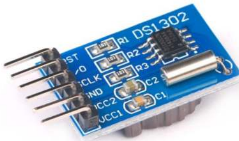
Figure 3.10 DS1302 Real-Time Clock (RTC) Module
