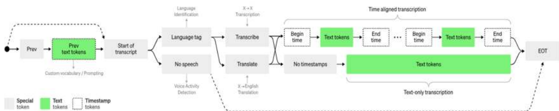
Figure 3.6 Phrase-level timestamps, multilingual speech transcription, and to-English speech translation
