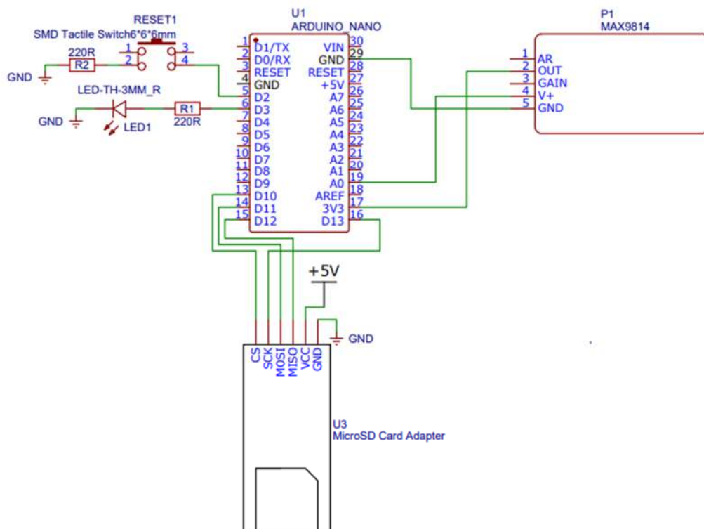
Figure 3.21 Hardware Circuit diagram
