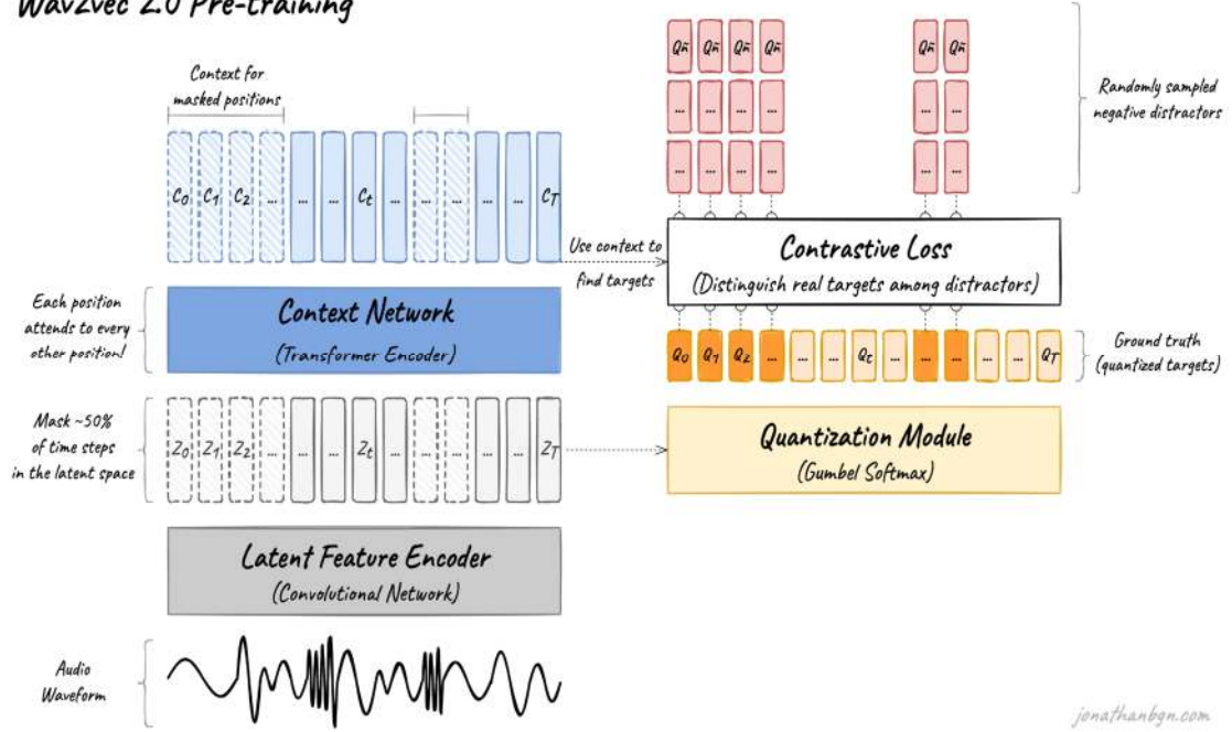
Figure 3.7 wav2vec 2.0 architecture and its pre-training process
