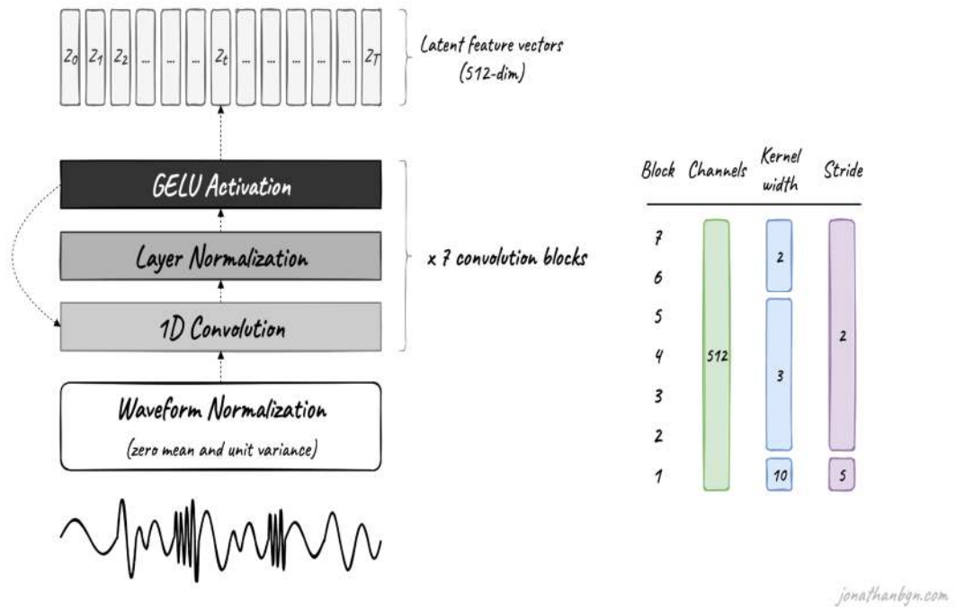
Figure 3.8 Wav2vec 2.0 latent Feature Encoder
